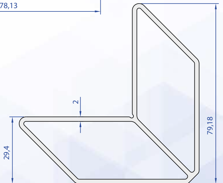
06954-00 1,673 Kg/m
