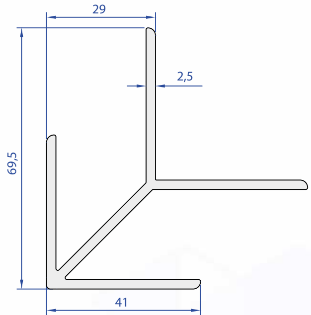
81008-00 1,325 kg/m
