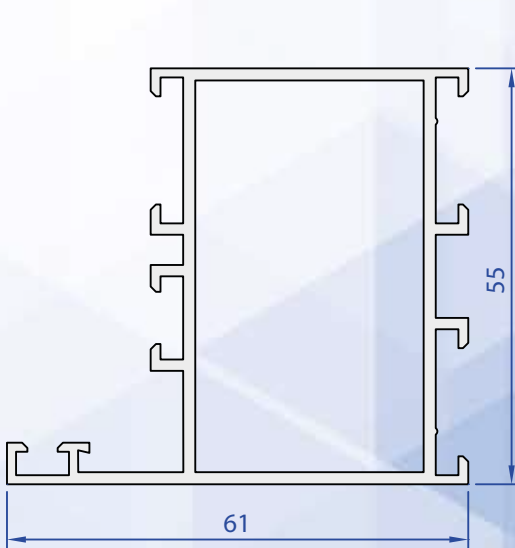
81009-00 1,073 Kg/m
