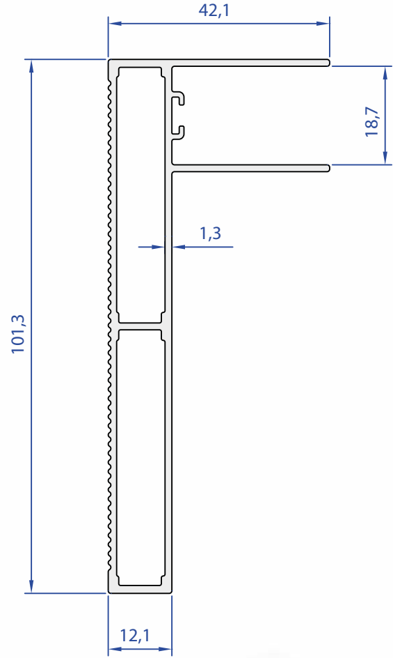
75354-00 1,093 Kg/m
