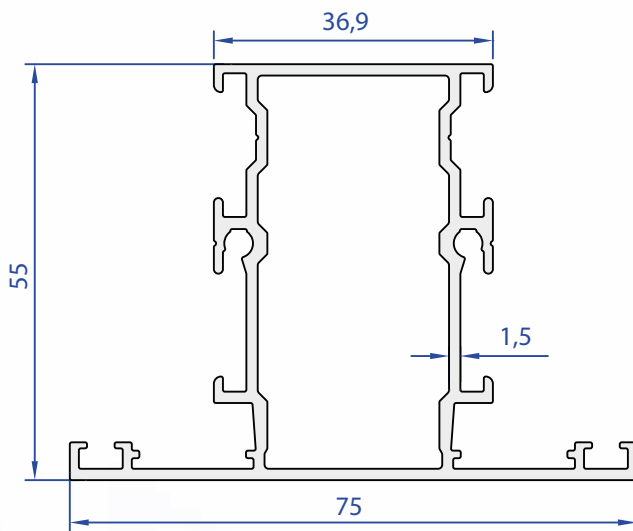
81007-16 1,138 kg/m
