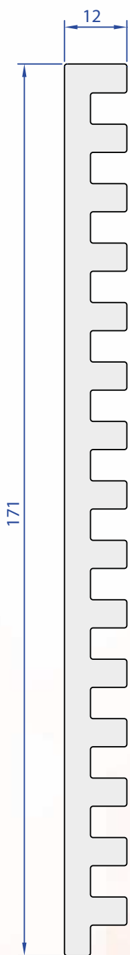
40242-00 3,856 Kg/m
