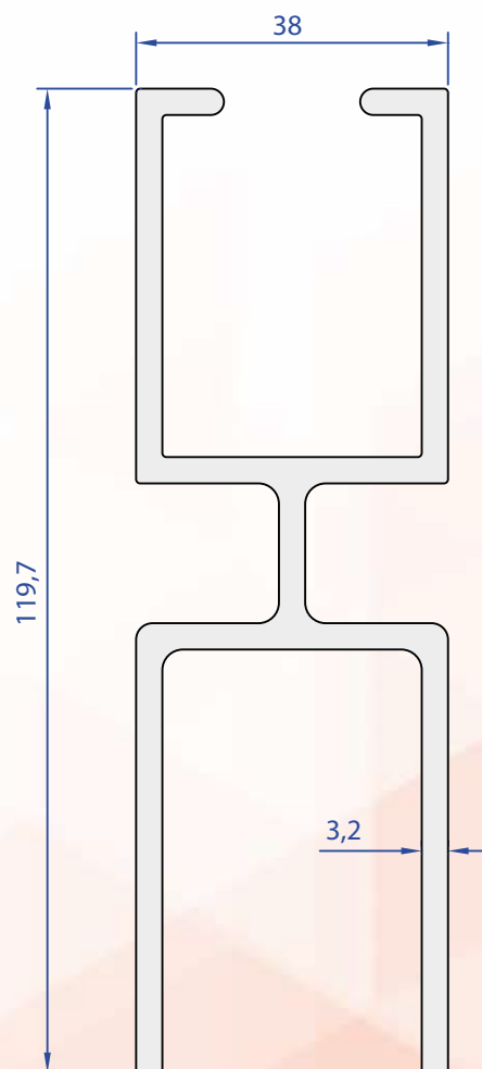
07198-00 2,617 Kg/m
