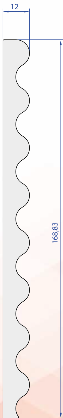
06505-00 4,066 Kg/m
