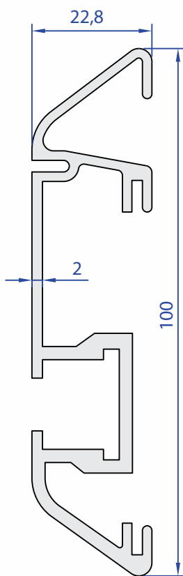
60008-00 1,375 kg/m
