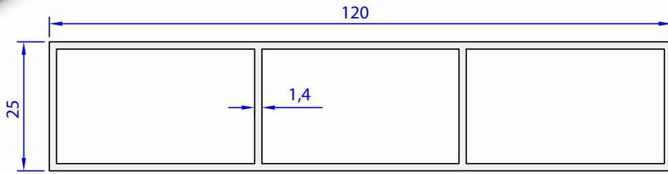
06495-00 1,247 Kg/m
