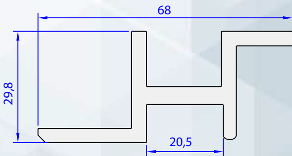
05174-00 1,293 Kg/m
